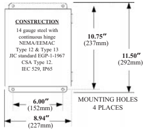
NEMA 4 / 12 enclosure.
